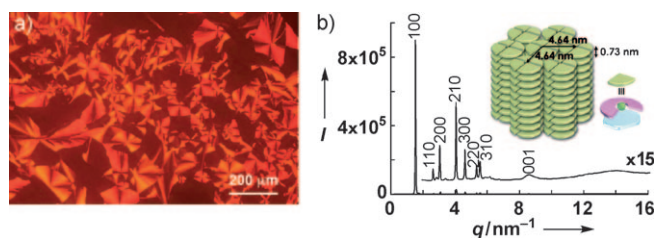
Figure 3. a) Polarizing optical microscope image of 2\text{-Cl}^-(\text{TATAC}^3)^+ at 87^\circ\text{C} by cooling at 2^\circ\text{Cmin}^{-1} from the isotropic liquid phase (Iso). b) XRD pattern of 2\text{-Cl}^-(\text{TATAC}^3)^+ in the mesophase at 70^\circ\text{C} after cooling from Iso and the proposed assembling model (inset). In-plane spacings: 4.64 nm; between layers: 0.73 nm.
